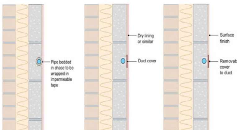
12. Accessibility of Pipes in Internal Walls
