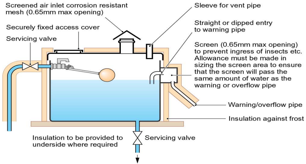
13. Details for Cistern Storing Water For Domestic Purposes
