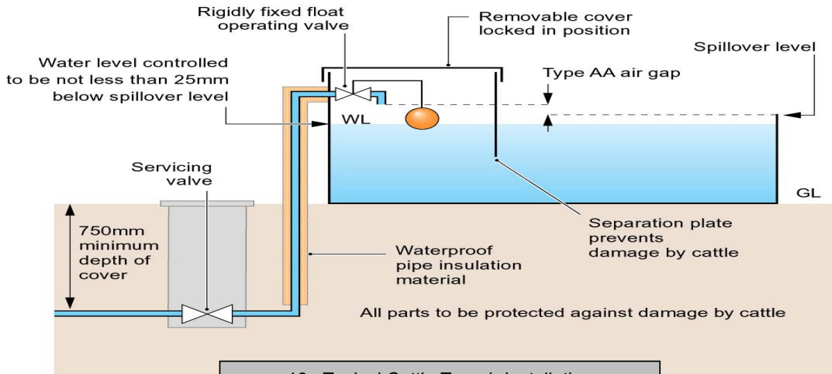
16. Typical Cattle Trough Installation
