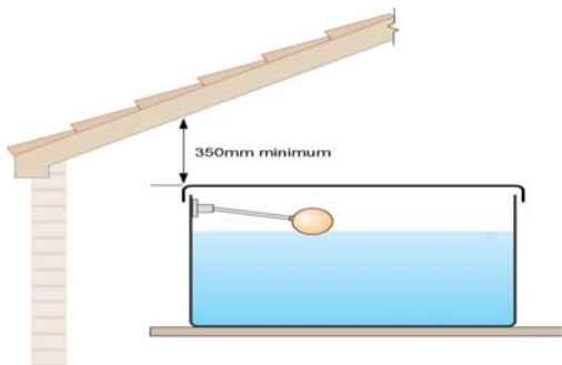
14. Minimum Unobstructed Space for Access to Cistern of 1000 Litres Actual Capacity or Less
