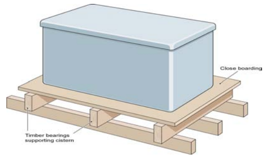
15. Example of Close Boarded Support to Plastic Cistern
