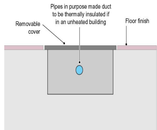
10. Accessibility of Pipes Laid in Solid Floors
