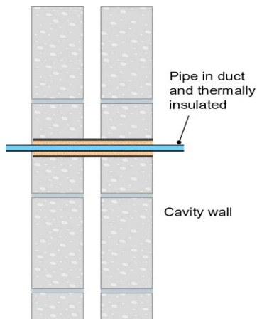
11. Pipes Passing Through Walls
