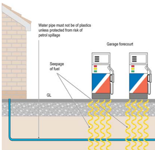
5. Protection of Plastic Pipes from Petroleum Products
