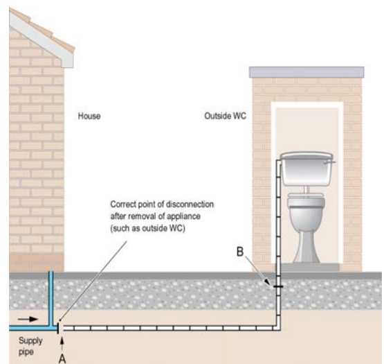
6. Sealing off Redundant Pipes
